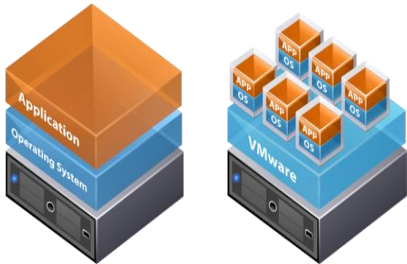
Virtual Machine
