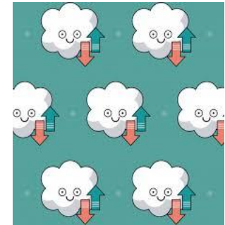
Storage Service
